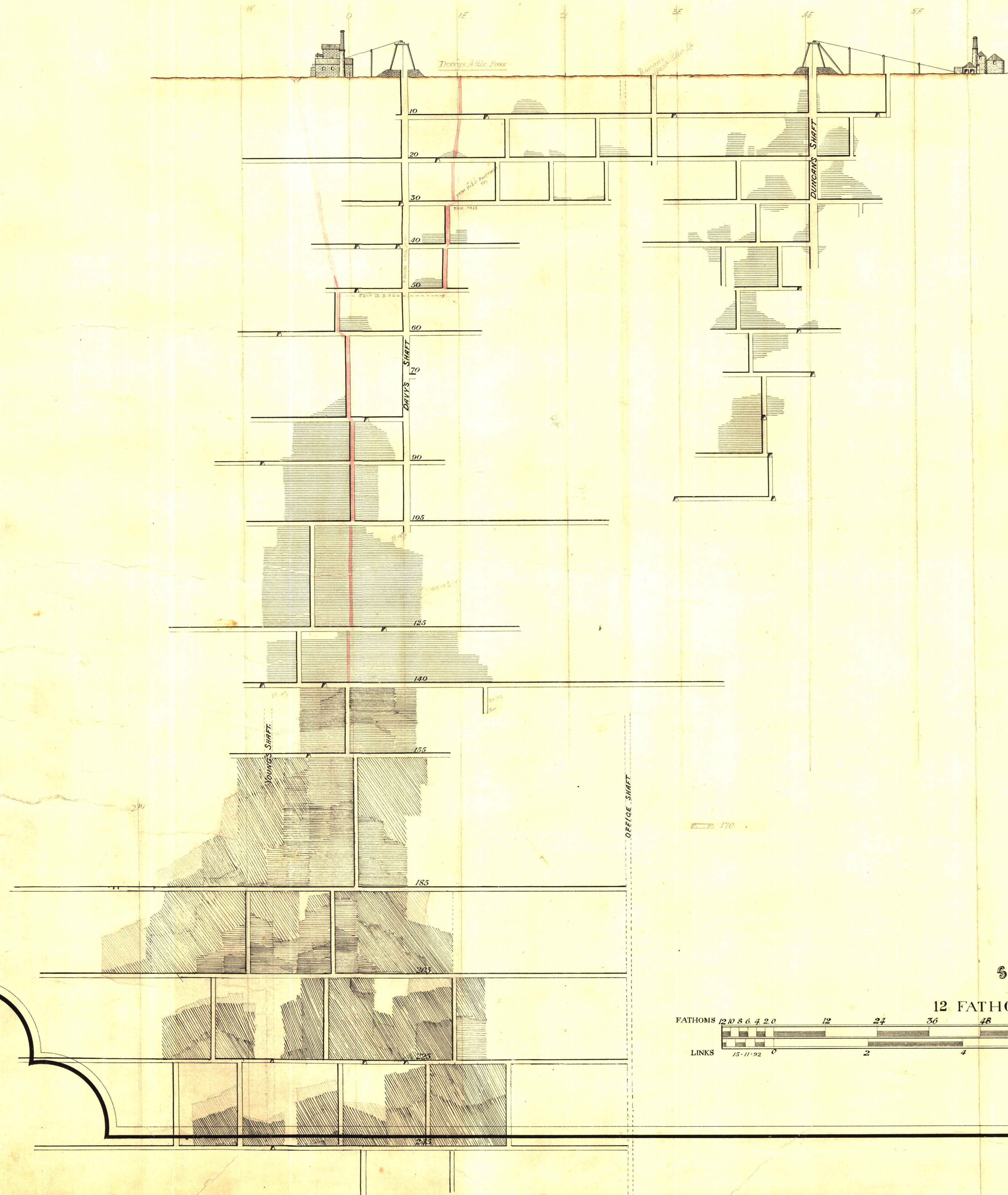
LONGITUDINAL SECTION OF NAVY'S LORE
