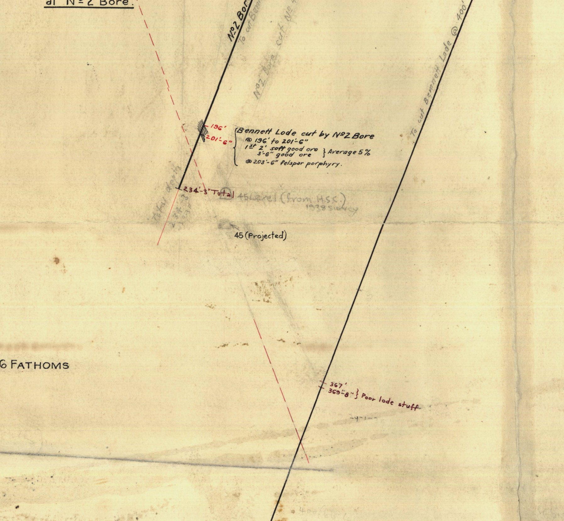
X Section thru' Bennett Lode at N°2 Bore.
